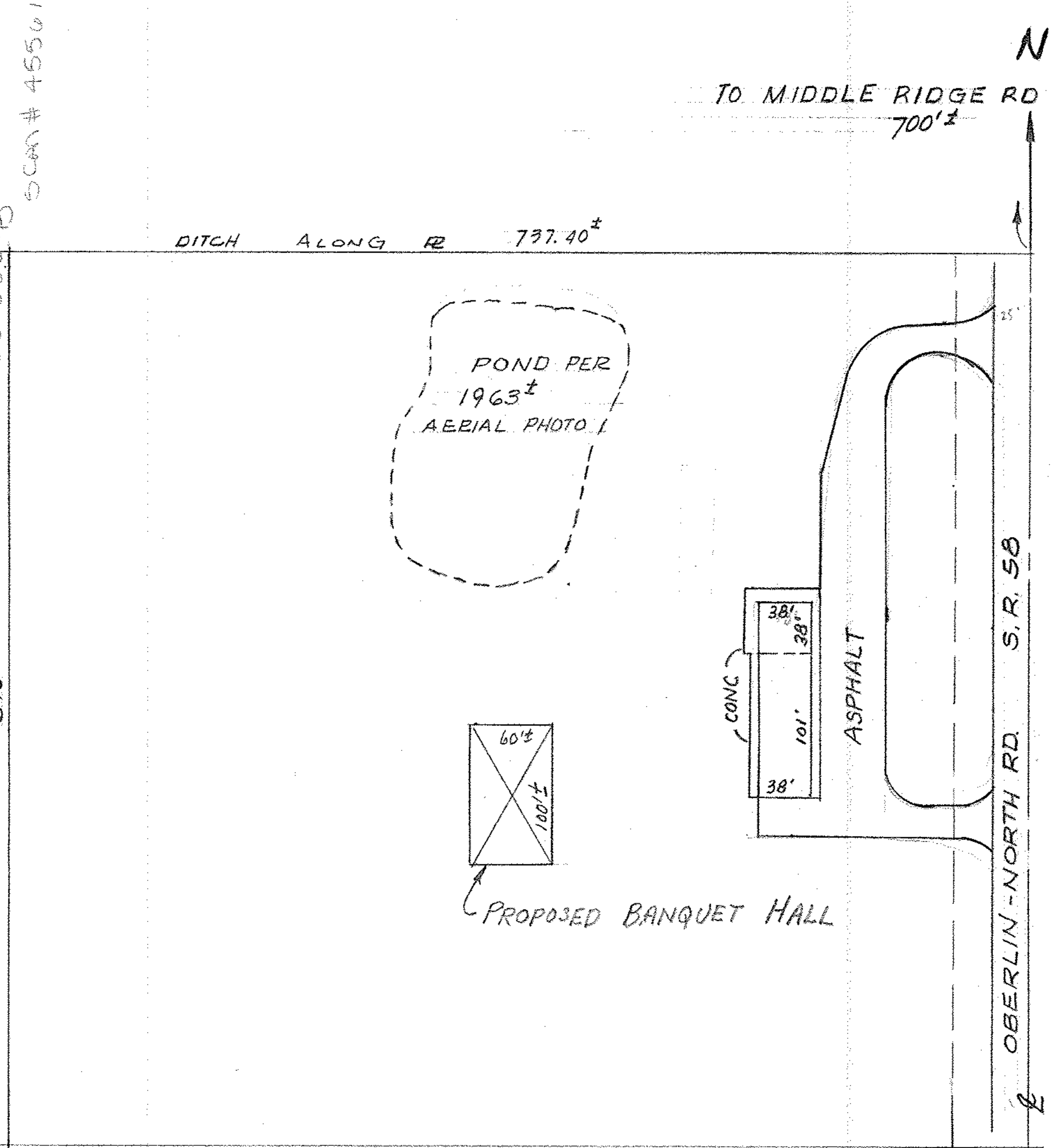
SITE LOCATION PLAN 1" = 100'±
