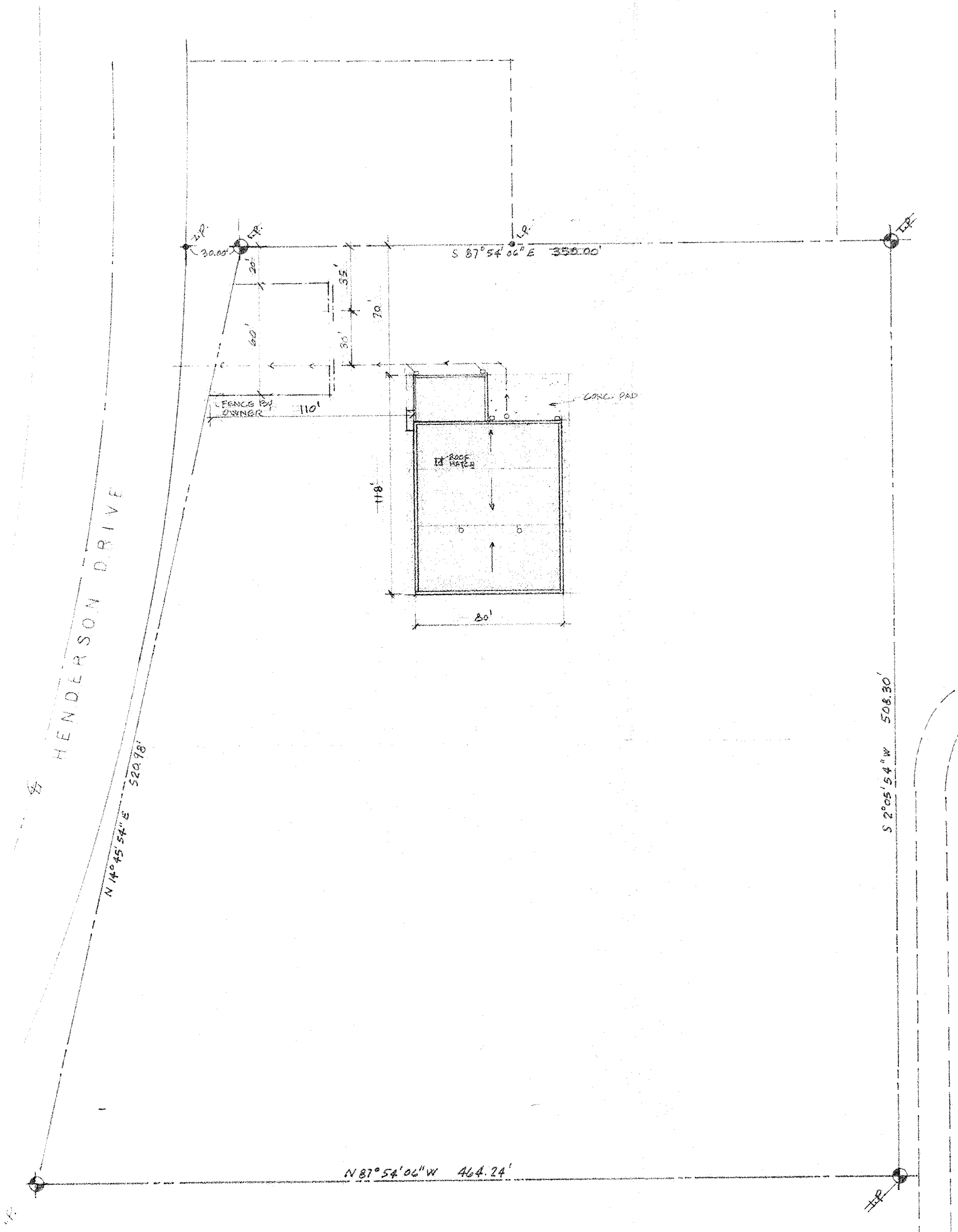
SITE PLAN SCALE - 1" = 40'
