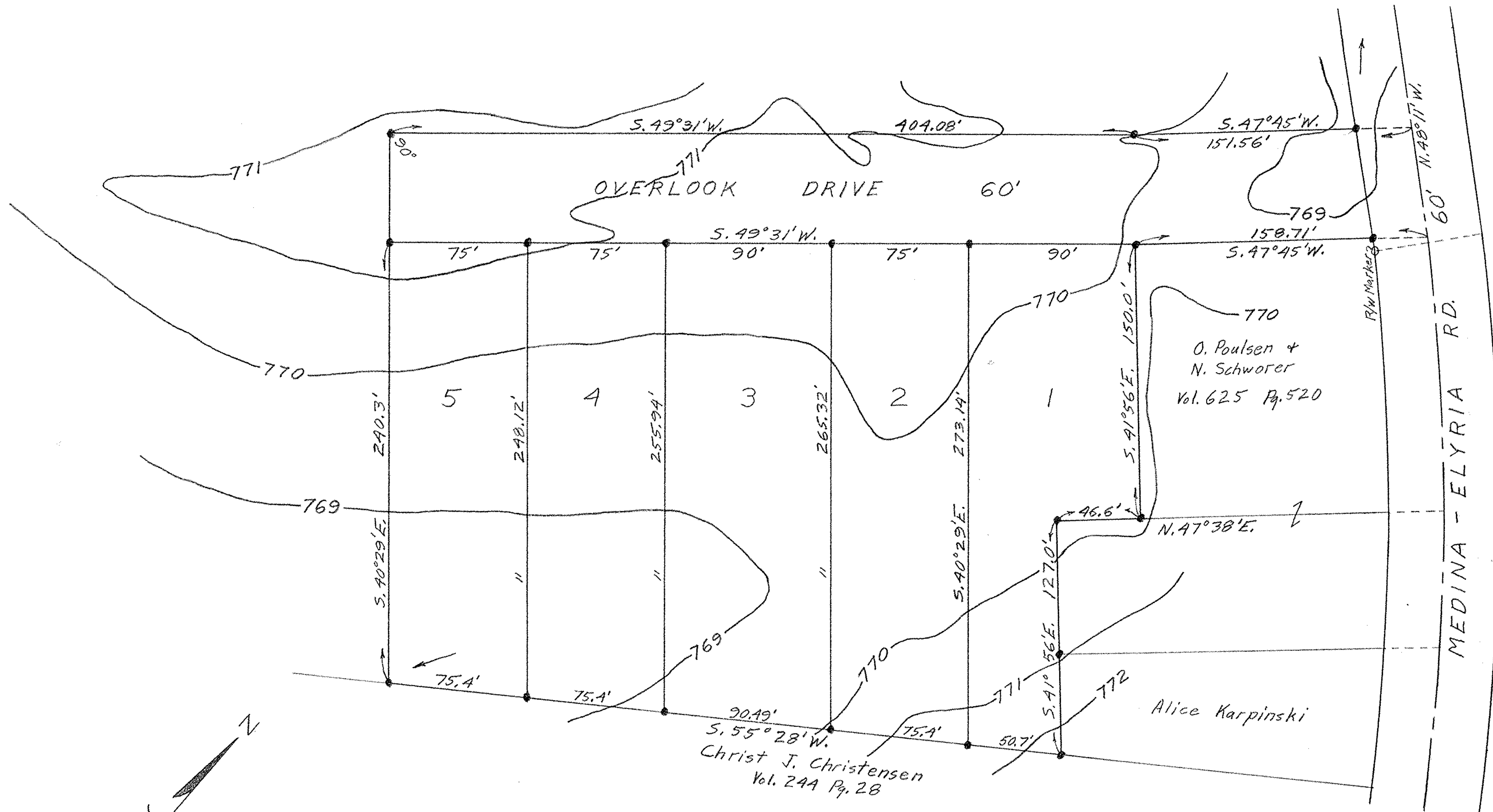
CONTOUR MAP OF PROPOSED POULSEN ALLOTMENT SECTION NO. 6 CARLISLE TWP. LORAIN COUNTY - OHIO SCALE: 1" = 50' MAY 8, 1956 C. E. Penfound Registered Surveyor
