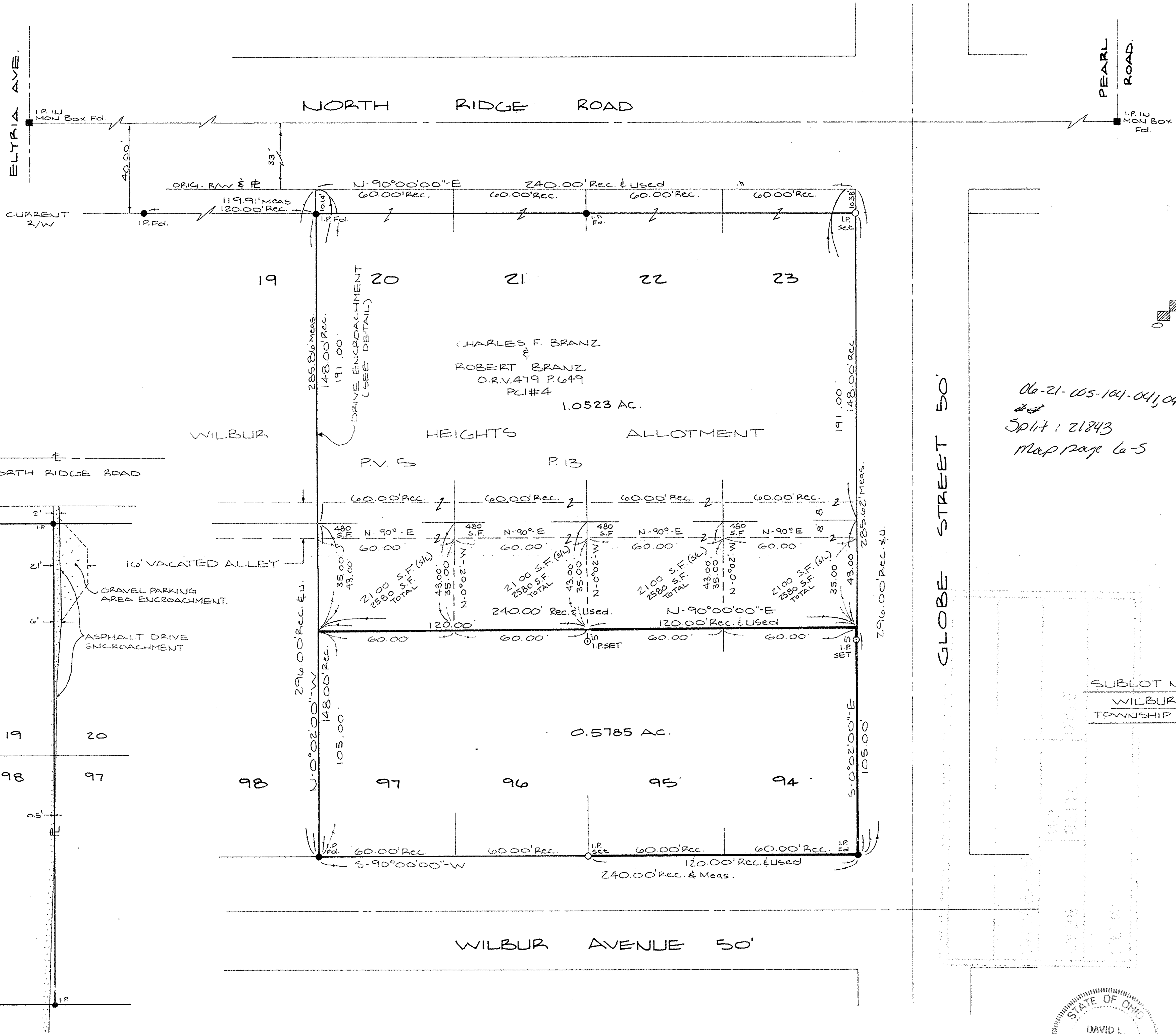
WILBUR AVENUE DETAIL SCALE: 1" = 40'
