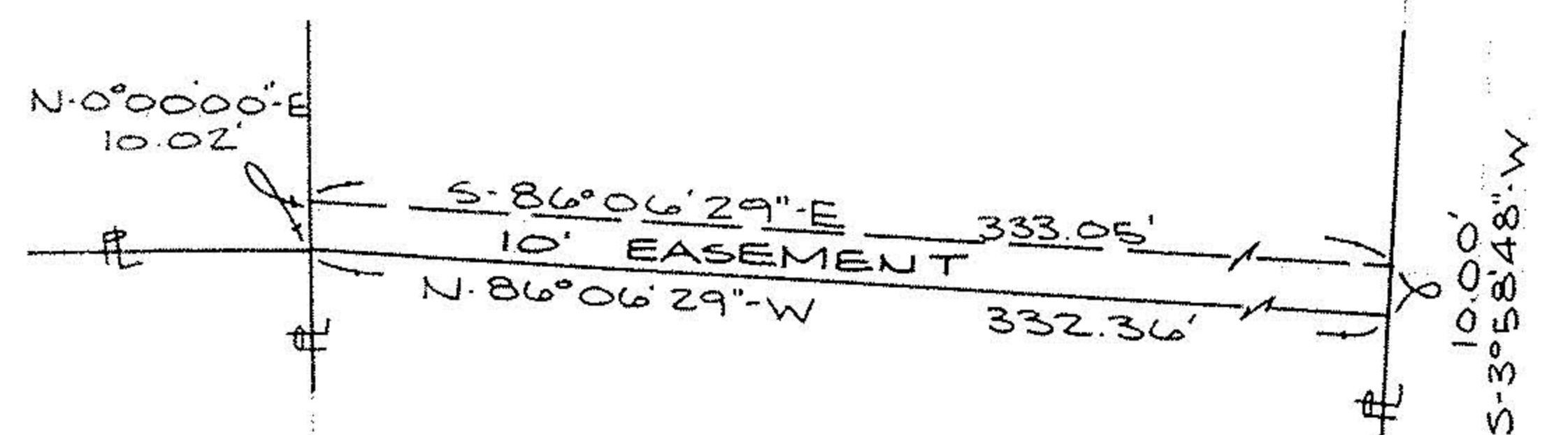
DETAIL EASEMENT SCALE: 1" = 60'
