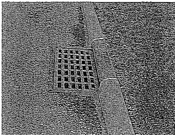
Example of bike-safe storm water inlet grates
