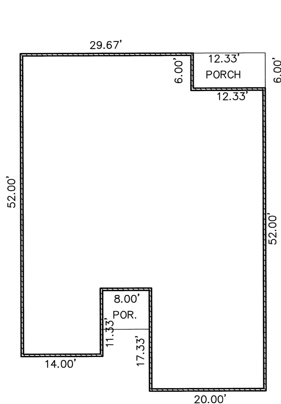
FOUNDATION PLAN (EXTERIOR DIMENSIONS)
