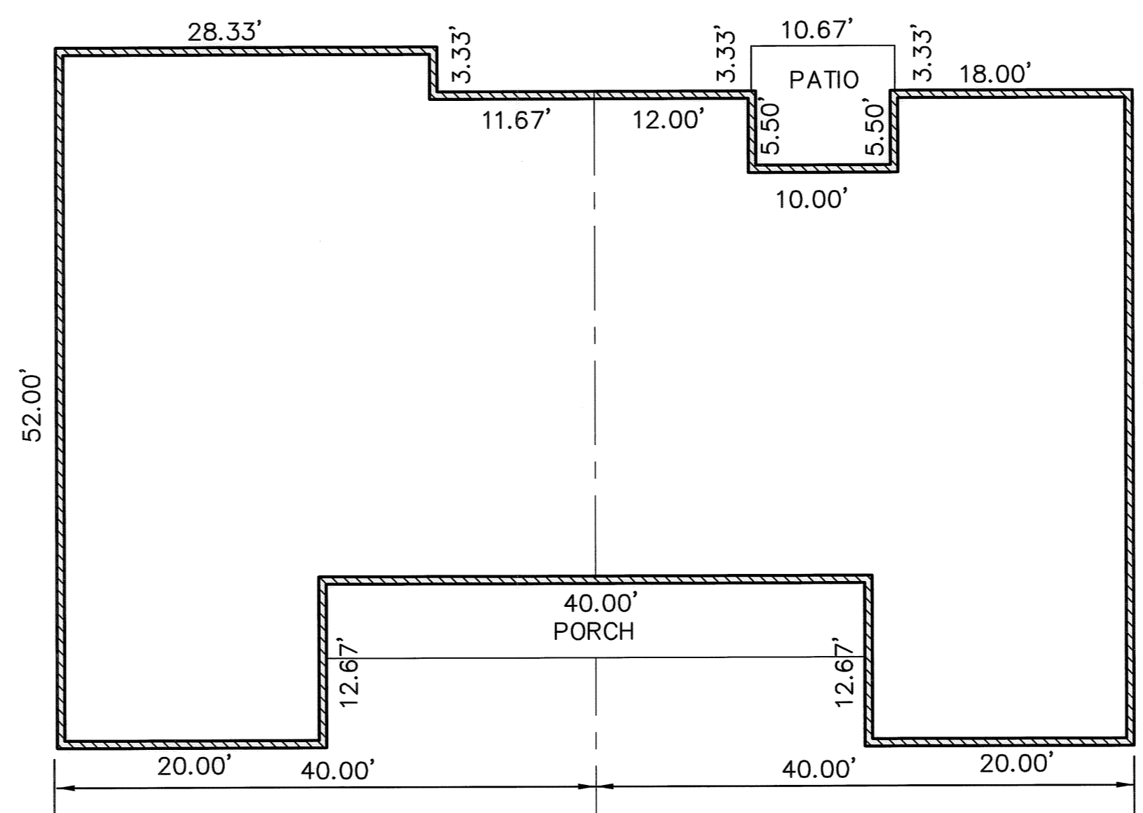
FOUNDATION PLAN (EXTERIOR DIMENSIONS)
