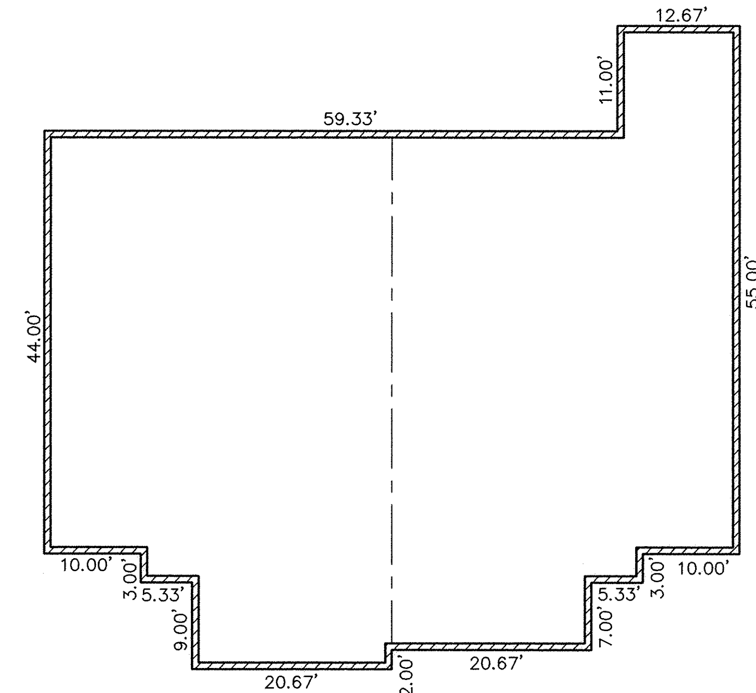
FOUNDATION PLAN (EXTERIOR DIMENSIONS)
