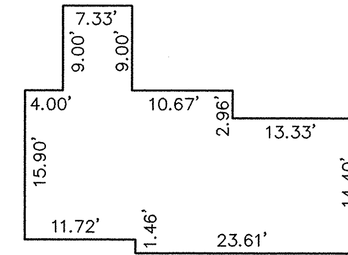
NOTE: TYPICAL FOR UNIT 97 REVERSE FOR UNIT 98 SECOND FLOOR PLAN (INTERIOR DIMENSIONS)
