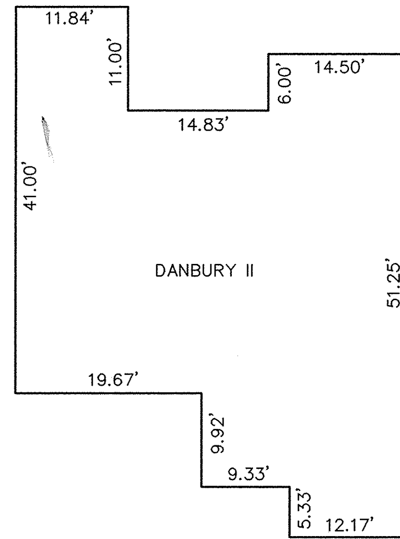
FIRST FLOOR PLAN (INTERIOR DIMENSIONS)
