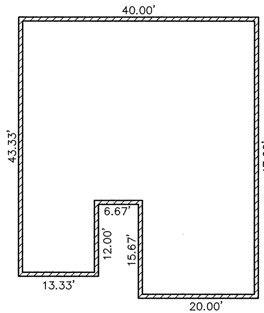
FOUNDATION PLAN (EXTERIOR DIMENSIONS)
