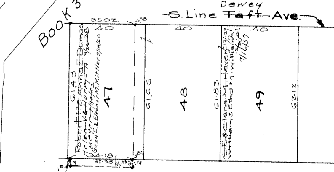
DETAIL Scale 1"=30'
